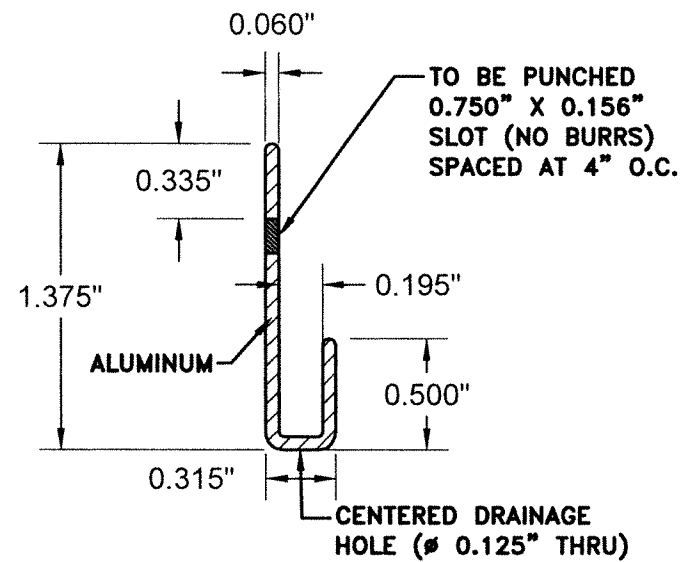
② EXTERIOR STARTER STRIP
