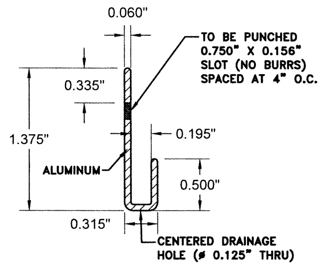
② EXTERIOR STARTER STRIP
