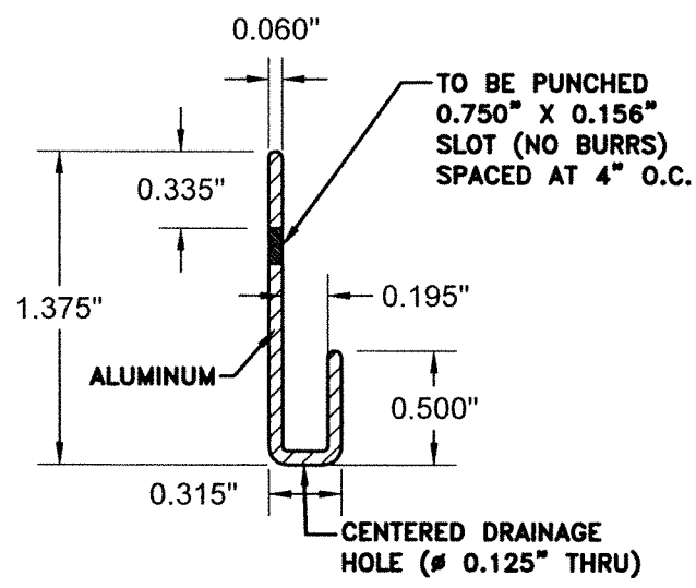
② EXTERIOR STARTER STRIP
