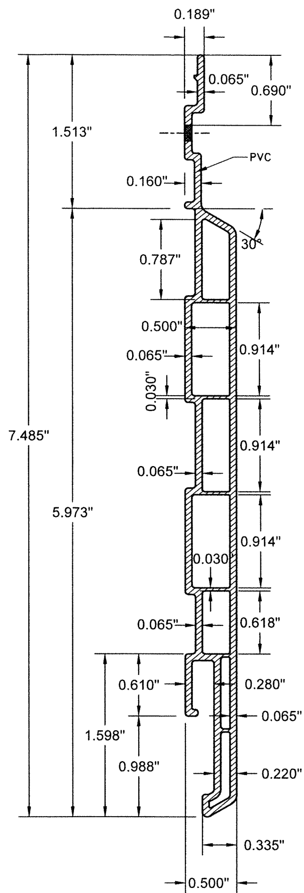
①A CWS 6" EXTERIOR 1/2" WALL PANEL W/ ⑩A OR ⑩B
