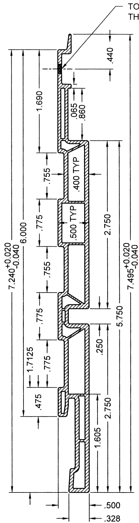
①C CWS 6" EXTERIOR 1/2" WALL PANEL W/ ⑦A OR ⑦B
