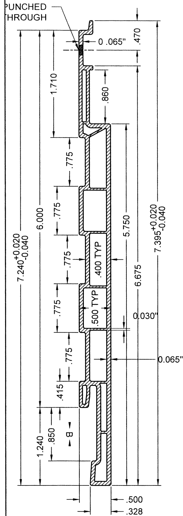
①B CWS 6" EXTERIOR 1/2" WALL PANEL W/⑩A OR ⑩B
