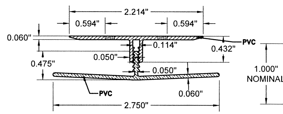
⑥ H-TRIM BASE & COVER CAP
