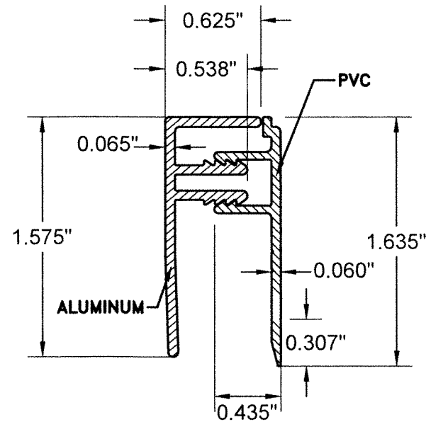
④ 6" SIDING 2 PC FINISH TRIM
